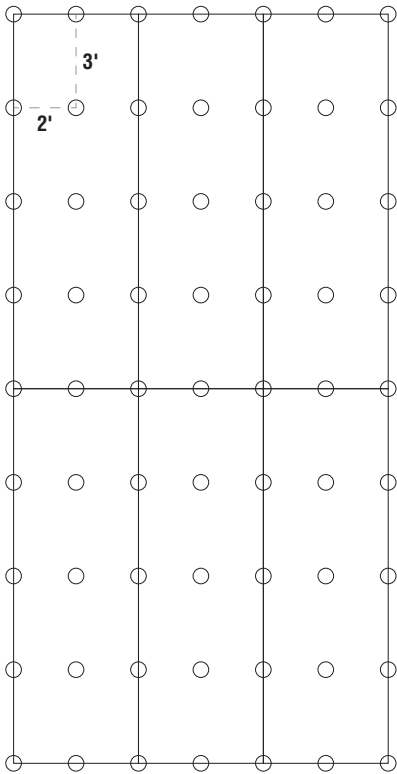
4' x 12' Panels
