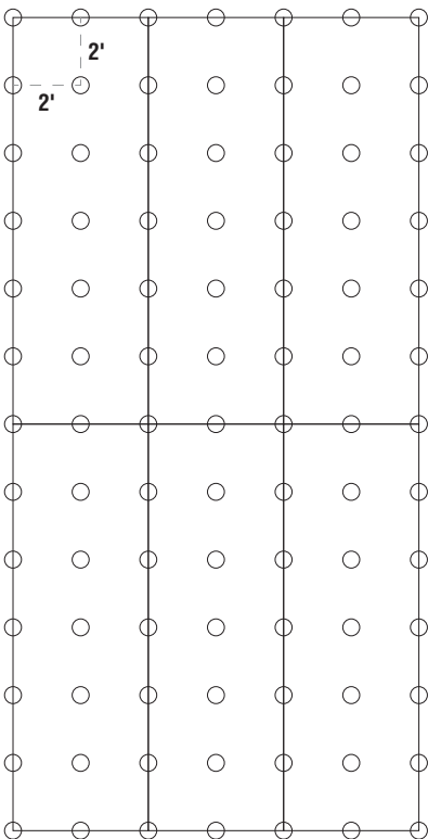
4' x 12' Panels
