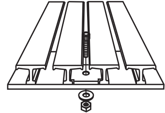
The weldable 316L stainless steel insert clips above are available for DURAGRID® T-1800 and T-3500 only. *Bolts are priced separately from the hold-down.
