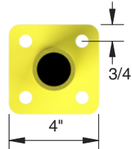
Post Base (Mounted To Post)
