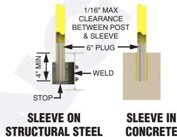
Removable Posts
