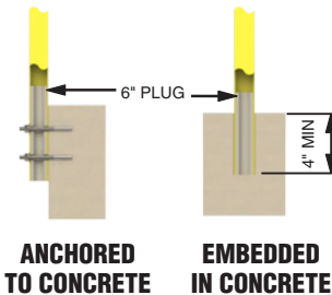
Fastening to Concrete
