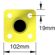
Post Base (Mounted To Post)
